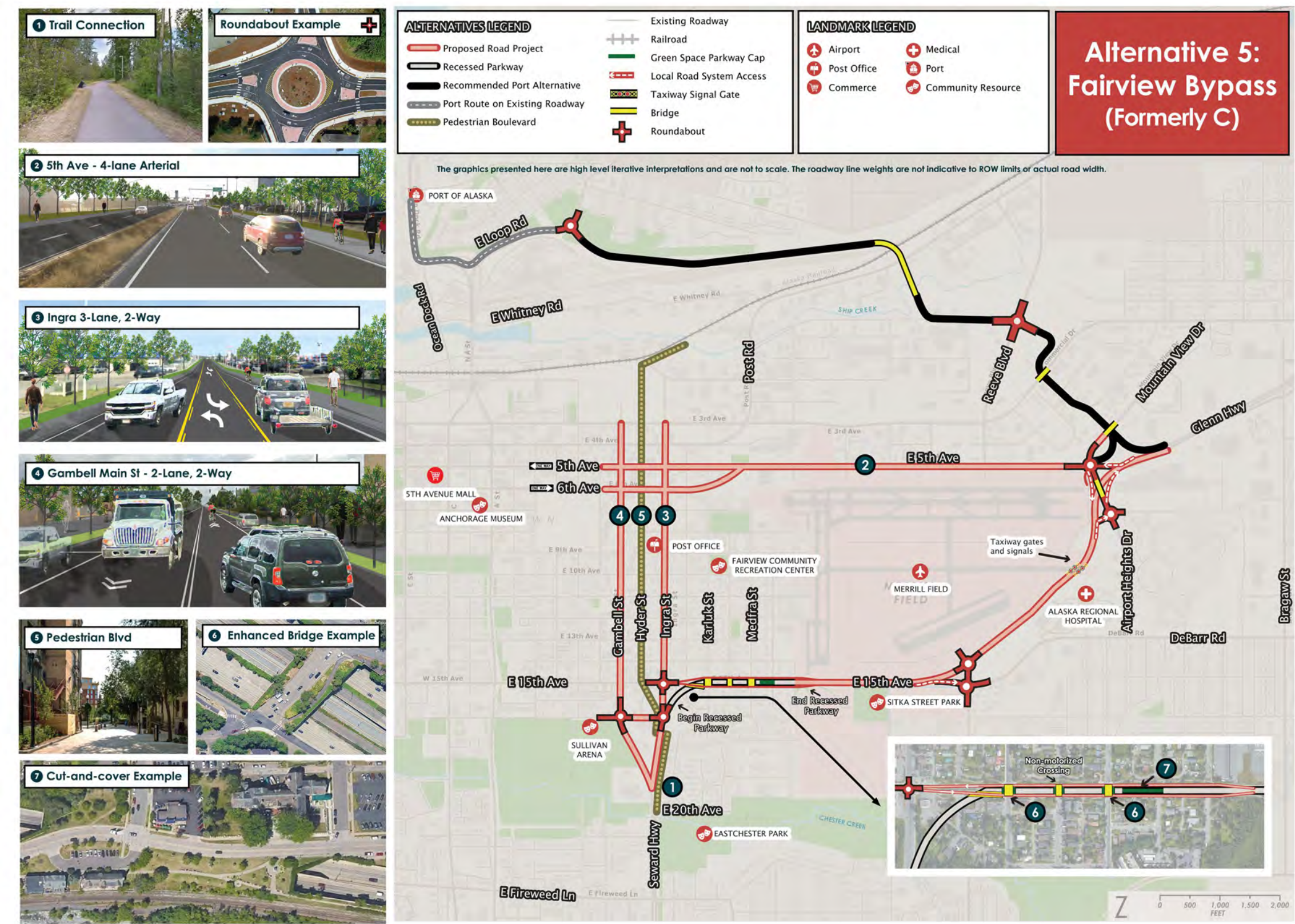
Figure 16. Alternative 5: Fairview Bypass
